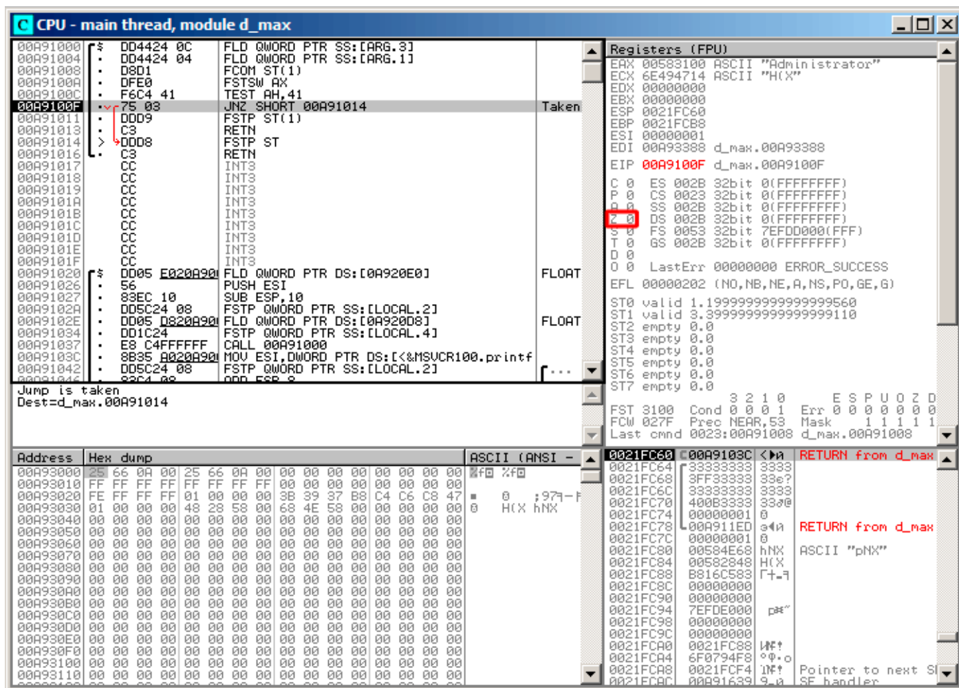
Figure 1.80: OllyDbg: TEST is executed
